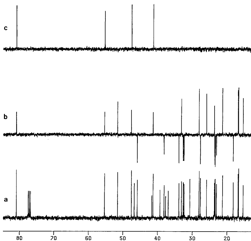
Fig. 2.2.1. ^{13}\text{C} DEPT spectra of 3-acetyloleanolic acid methyl ester, aliphatic region only: a broadband ^1\text{H} decoupled spectrum;
