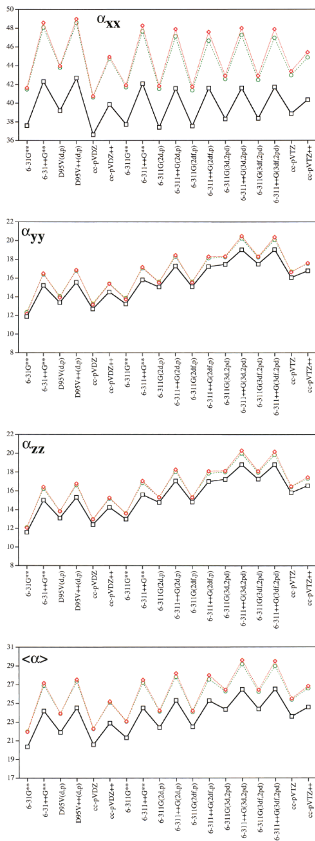
Figure 1. Theoretical level dependency of the atomic polarizability tensor components \alpha_{xx} , \alpha_{yy} , and \alpha_{zz} and the isotropic polarizability \langle\alpha\rangle of carbodiimide. RHF data are marked by squares and connected by solid lines, MP2 data are marked by diamonds and connected by dotted lines, and QCISD data are marked by circles and connected by dashed lines. Units are in \text{au}^3 .
