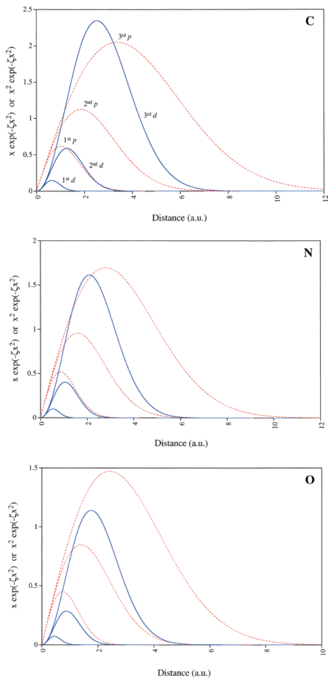
Figure 2. Radial distribution functions x \exp(-\xi_i x^2) (dashed) and x^2 \exp(-\xi_i x^2) for the p- and d-type primitive functions of C, N, and O (top to bottom). The exponents \xi_i employed are those of the 6-311+G(3d) basis sets.
