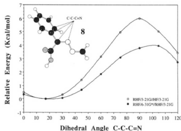
Figure 7. Rotational profiles for phenyl rotation in the model system HOCCPh=NNCH 2 , 8, with \tau = 180^\circ as a function of the dihedral angle C (syn,ortho) -C-C=N.
