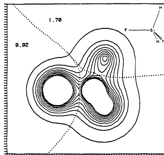
Figure 3. Contour representation of the projection function for fluorosilane at the 3-21G* level. Contours from 0.01 to 0.51 with a gradient of 0.05 \text{ e au}^{-2} . Dotted lines demark regions integrated for IPP analysis.
