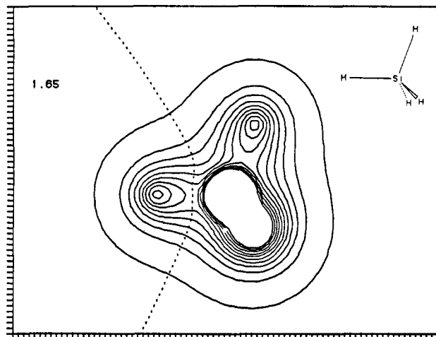
Figure 1. Contour representation of the projection function for silane at the 3-21G* level. Contours from 0.01 to 0.51 with a gradient of 0.05 e au -2 . Dotted lines demark regions integrated for IPP analysis.
