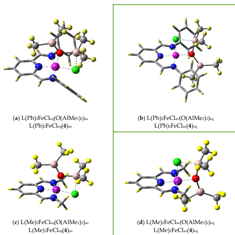
Figure 4. Computed structure of catalyst with the Sinn monomer 4 , \text{O}(\text{AlMe}_2)_2 a small acyclic aluminoxane. Top row: N,N -diphenyl ligand L; bottom row: N,N -dimethyl ligand L. Left column: equatorial chloride; right column: axial chloride.
