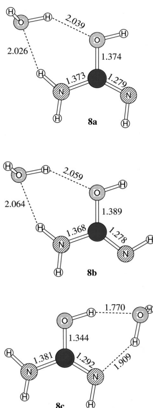
Figure 7. MP2(full)/6-31G* optimized structures for the three possible hydrated isourea intermediates in the two-water hydrolysis of carbodiimide. Structures 8a and 8c are E-configured about the C=N bond and structure 8b is Z-configured.
