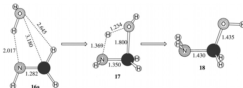
Figure 12. \text{MP2}(\text{full})/6-31\text{G}^* optimized structures for the one-water hydrolysis of methyleneimine.
